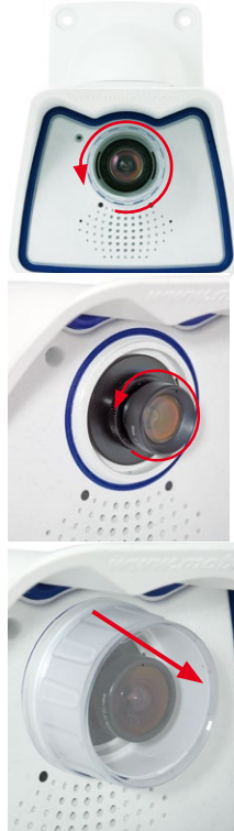
Lock ring
